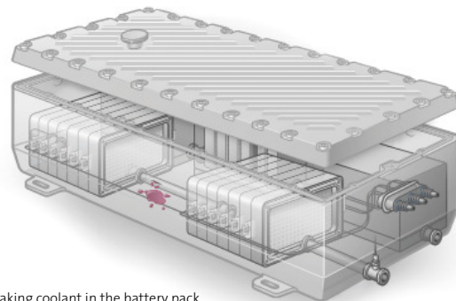
Leaking coolant in the battery pack
