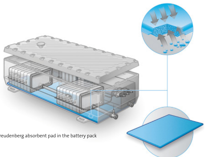
Leaking coolant in the battery pack
